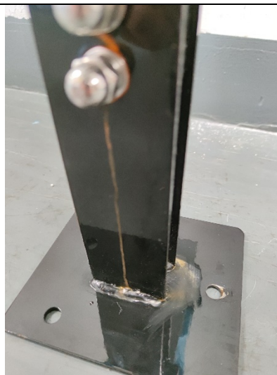
After 150 hours test - View 6
