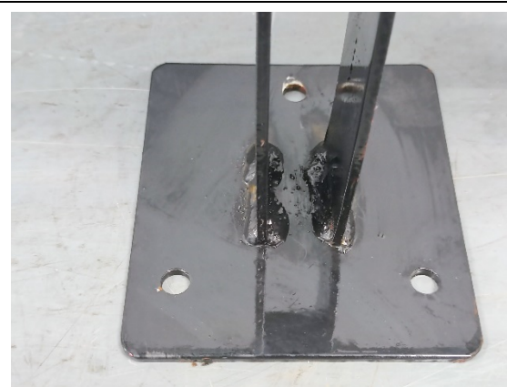
After 240 hours test - View 16
